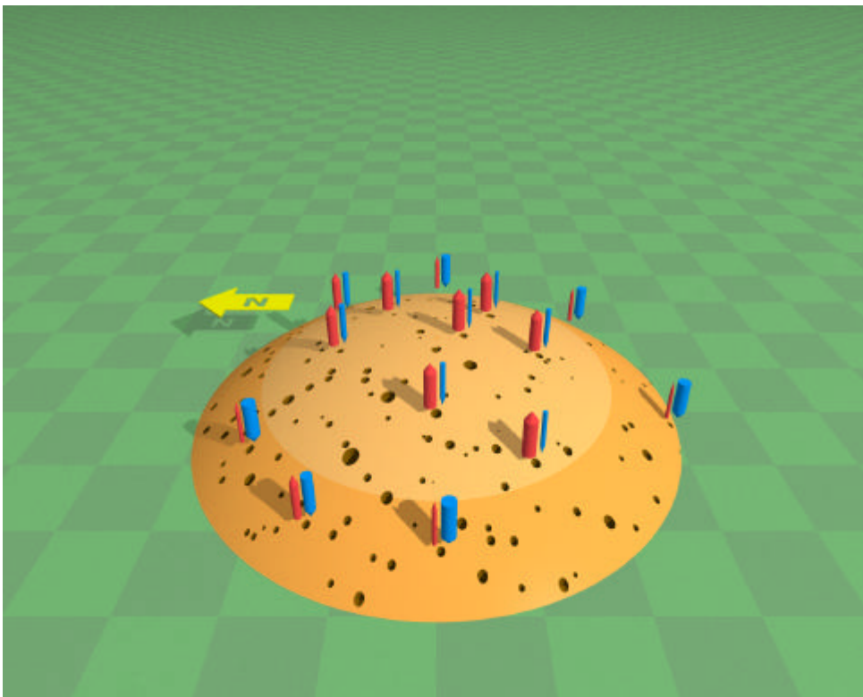
Schematic drawing of a nest mound of Atta vollenweideri . The arrows indicate the probability of inflow (blue) and outflow (red).
