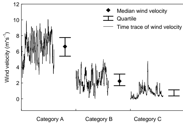
Fig.2.2 Decreasing wind velocity during one long-term recording was used to assign three different wind categories which were used to analyze the dynamics of nest ventilation.
