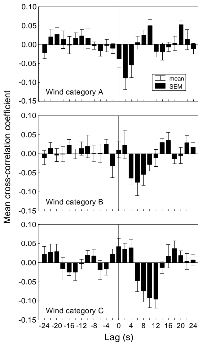
Fig.2.8 Phase relation of inflow channels to outflow channels at the three different wind categories. For cross-correlation the first derivatives of the air velocities were used. Each data set of the two outflow-channels was cross-correlated with each data set of the three inflow channels.
