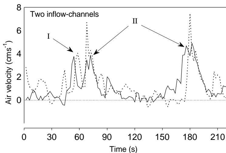
Fig.2.9 Example of air velocity in two different inflow-channels during a period of 210 s. Inflow does not occur simultaneously in two different inflow-channels and no consistent phase relation between these two channels exists during the three analyzed time sections of 20 min. As in Fig.2.6, positive values denote inflow.
