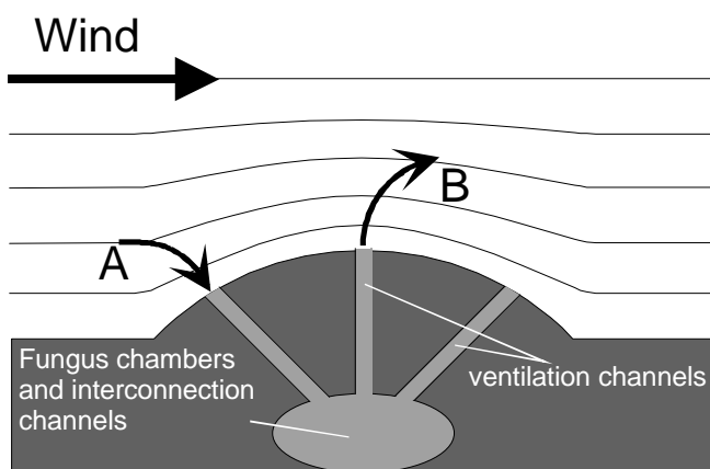
Fig.2.1 Schematic cross section through a nest of Atta vollenweideri with indication of possible ventilation mechanisms. Wind might pump air into channels on the upwind side (A) and/or might suck out air through central channels (B).
