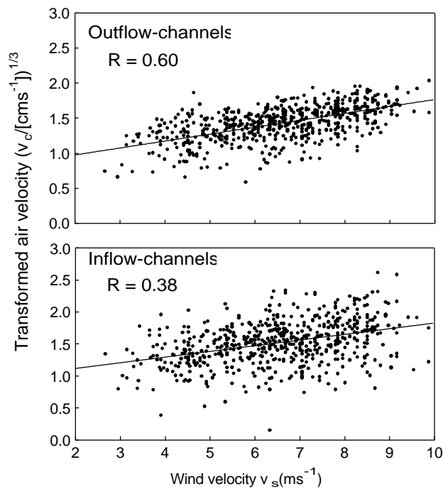
Fig.2.7 Correlation between surface wind velocity and air velocity (transformed values) in two outflow-channels (upper, pooled) and three inflow-channels (lower, pooled). The slopes of both regressions are not significantly different. Note the higher correlation of outflow-channels to surface wind.
