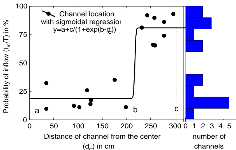
Fig.2.5 Inflow probability as a function of distance from the center of the nest (left). A sigmoidal regression describes more than 90% of the variance and the inflection point marks the border between inflow-channels at the periphery and outflow-channels in the center. Number of channels with respect to their inflow probability (right). Two distinct groups resembling inflow- and outflow-channels can be discriminated statistically.
