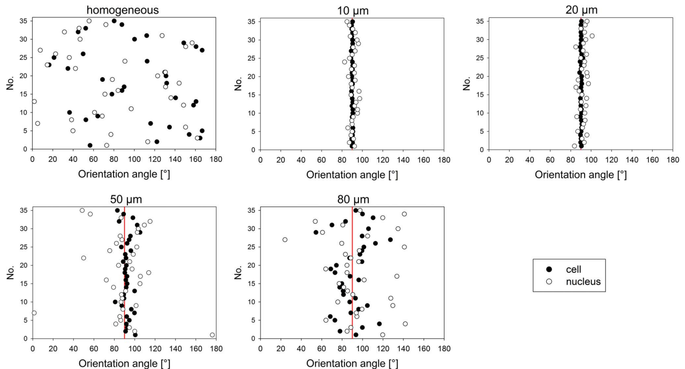
Figure 4. Alignment of cells and nuclei on various line dimensions. Orientation angle (ranging from 0^\circ to 180^\circ ) was measured using a horizontal line as reference line. On micro-patterned substrates, orientation angle of stripes was 90^\circ (indicated by red lines). On 10\ \mu\text{m} and 20\ \mu\text{m} lines, the orientation of cells and nuclei followed strictly the orientation of micro-patterned lines. These effects were less pronounced on 50\ \mu\text{m} and 80\ \mu\text{m} lines. On homogeneously functionalized fibronectin substrates, both cells and nuclei were randomly oriented with no preferred direction. doi:10.1371/journal.pone.0109411.g004
