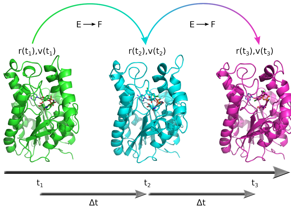
Figure 2.8 Schematic illustration of an MD simulation. For each time step \Delta t , the atomic position \mathbf{r}(t_i) and velocity v(t_i) is evaluated for every atom i . The underlying forces F_i are derived from the energy function of the molecular mechanical force field. Figure adapted from [102].
