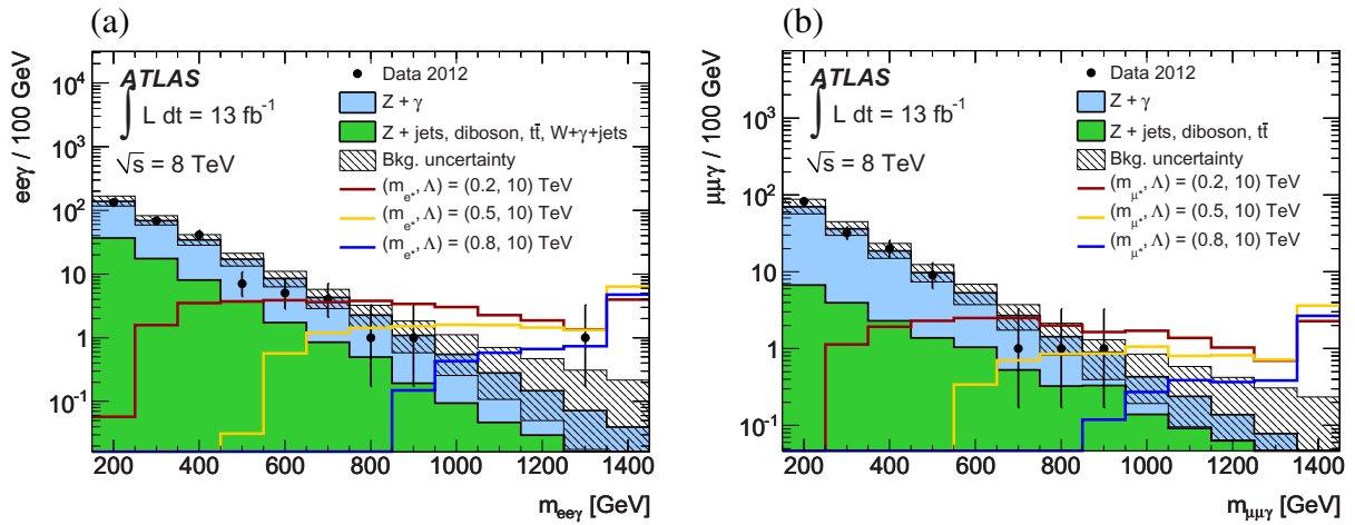
Figure 4. Distributions of the ll\gamma invariant mass ( m_{ll\gamma} ) for the electron (a) and muon (b) channels after requiring the dilepton mass to satisfy m_{\ell\ell} > 110 GeV. The binned results of exponential fits are used for the Z + \gamma , Z + \text{jets} , t\bar{t} and W + \gamma + \text{jets} backgrounds. The background uncertainty combining the statistical and systematic uncertainties is displayed as the hatched area. The last bin contains the sum of all events with m_{ll\gamma} > 1350 GeV. Signal predictions for three different values of the excited-lepton mass ( m_{\ell^*} ) with a compositeness scale ( \Lambda ) of 10 TeV are also shown.
