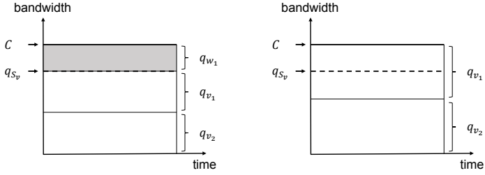
(a) FBV: Video flows share reserved data rate.
