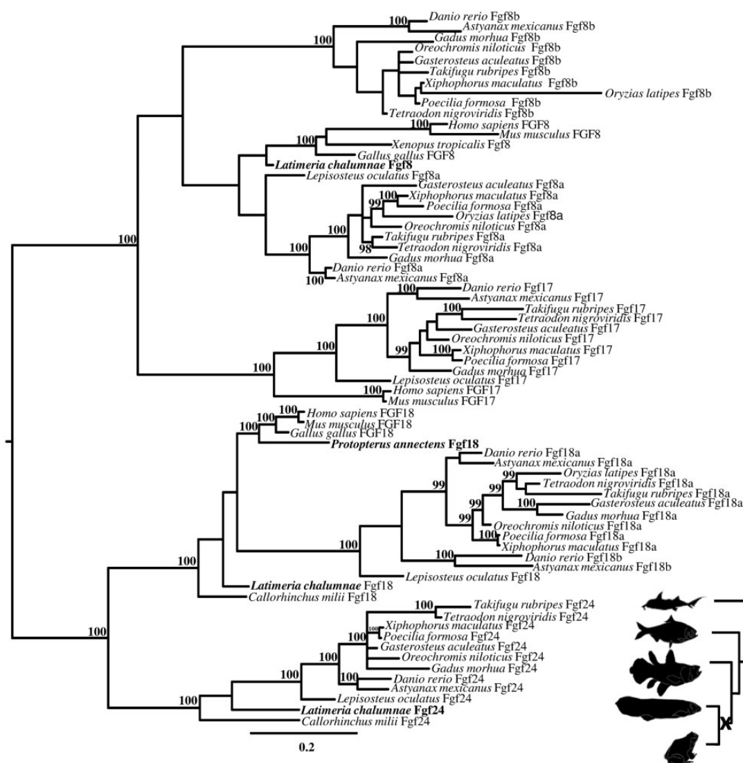
Fig. 4. —Fgf8/17/18/24 phylogeny. Phylogenetic analysis of Fgf8, Fgf17, Fgf18, Fgf24. Bayesian inference: 2,000,000 generations, sampling every 100, Jones substitution model, stationarity defined as when the average SD of split frequencies approaching 0.0062, burn-in set to 5,000, midpoint rooting. Numbers close to nodes indicate posterior probability values. Only values >95 were reported. The sequences in bold were obtained in this work.
