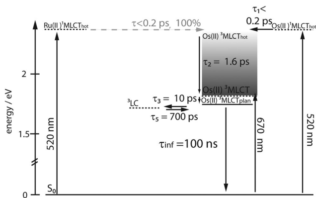
Scheme 2 Proposed relaxation scheme for RuOs , solid lines define energy levels with defined energetic positions, while dashed lines define excited states, the energy of which can only be indirectly inferred or depends on the excitation wavelength, processes in grey are not directly observable in the data.
