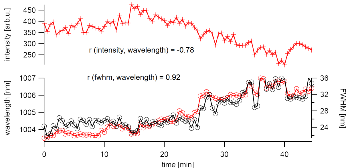
Fig. 55: Bleaching of the photoluminescence at 70\mu\text{W} laser excitation strongly correlates with peak broadening and a shift to lower energy. The bleach happens on a rather rapid time scale with a half-life decay of \tau=10\text{min} .
