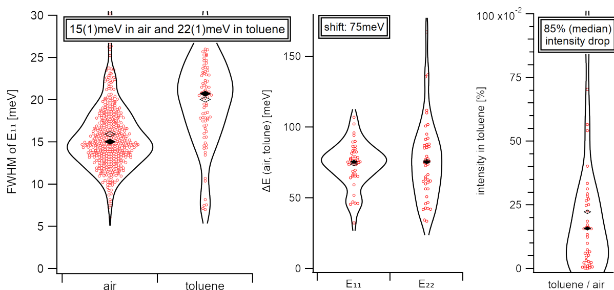
Fig. 16: The overall FWHM of the E 11 peak increases from 15meV (median) in air to 22meV (median) in toluene (left). This peak broadening is accompanied by a shift of 75meV to the red for both, E 11 and E 22 (middle). In toluene, the intensity drop drops to 15% (median) while the distribution maximum is more likely to be at around 5%. The distribution is shown as violin plot which is similar to a symmetrical histogram.
