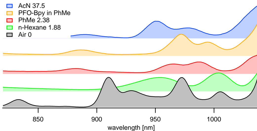
Fig. 29: The excitonic emission in toluene with adsorbed PFO-Bpy is shifted to the red compared to the emission in pure toluene. The graph shows the unweighted spectral autocorrelation of individual measurements.
