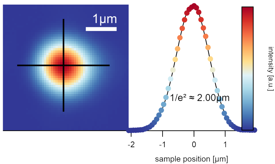
Fig. 45: The laser profile of the SuperK after the fiber output is around 1.2\text{mm} broad. If focused on the sample with the objective, it illuminates the area with a diameter of 2\mu\text{m} (the diameter of the laser spot is measured where the maximum intensity I_0 drops to I_0/e^2 ).
