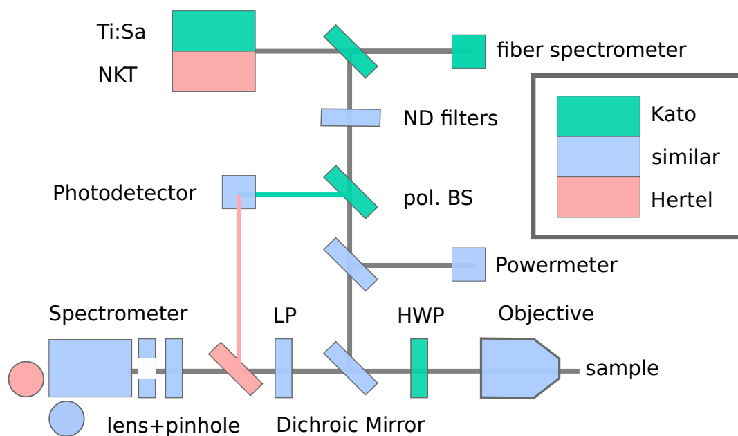
Fig. 31: Devised principal setup with emphasized similarities to the setup of the Kato group [136].
