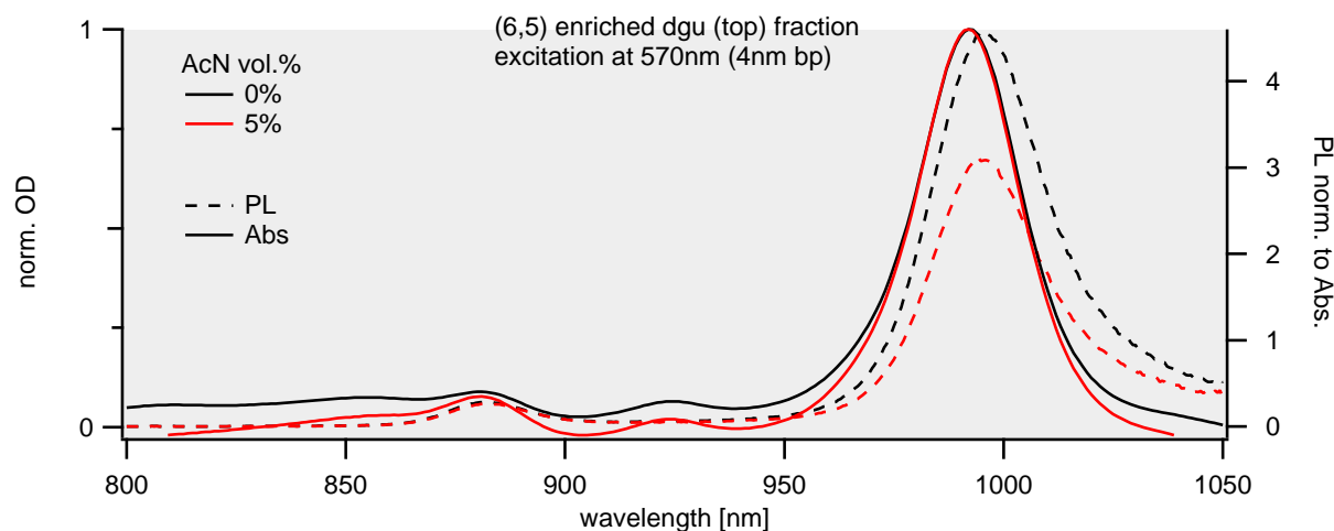
Fig. 28: Purified samples of the (6,5) type do not show a significant difference in their excitonic energy but also show a decrease in quantum efficiency
