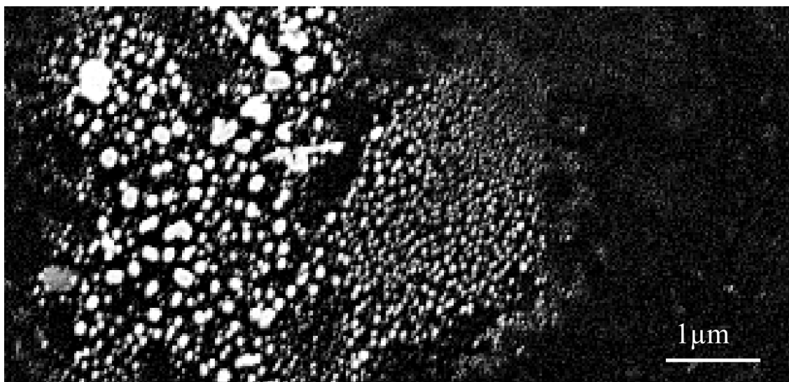
Fig. 20: Co-Rh catalyst particles on a silicon substrate after Oswald ripening under a hydrogen atmosphere at 600°C. The picture shows a spot with a large variety of particle diameters. Due to the high catalyst density in this area, Oswald ripening is producing particles up to 200nm in diameter.
