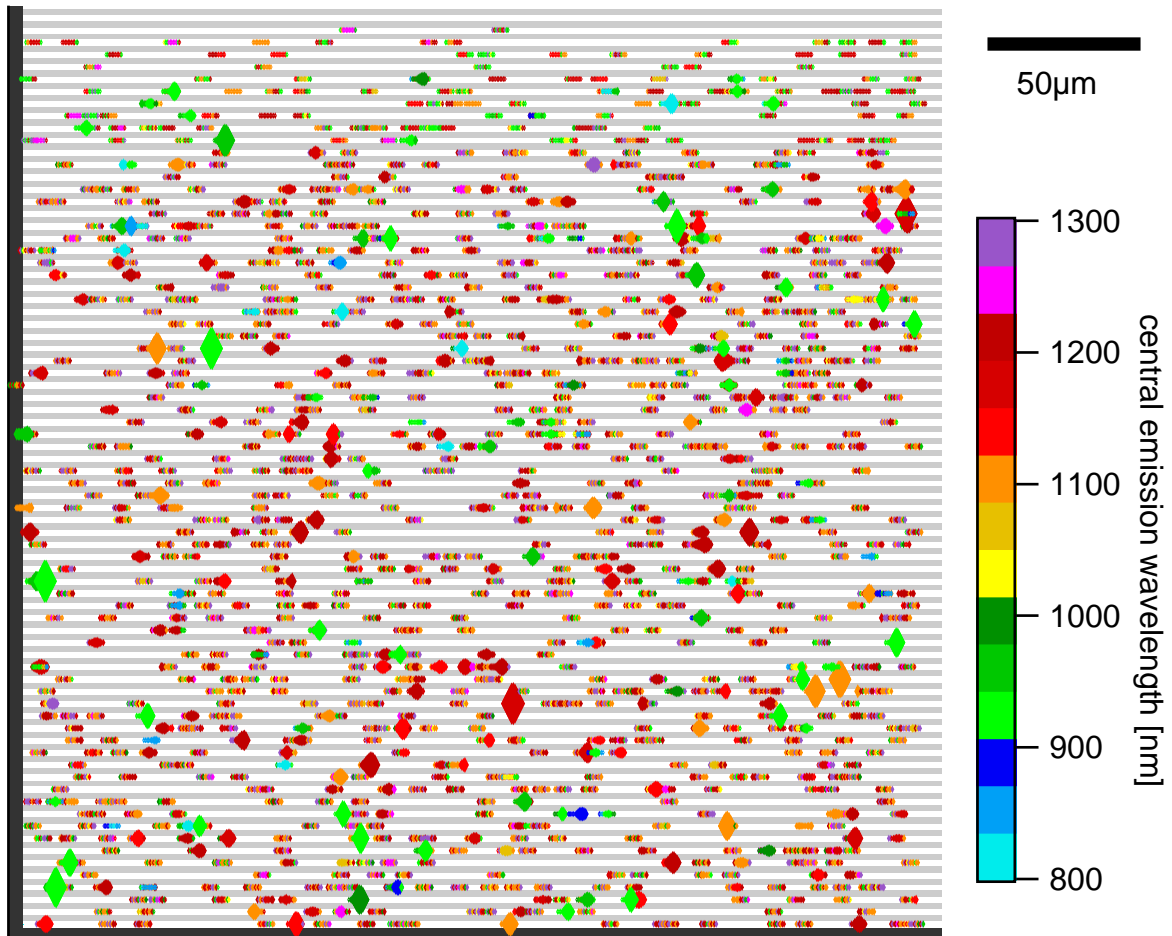
Fig. 56: The exact scan technique allows us to fully characterize, a sample area of 300\mu\text{m}\times 300\mu\text{m} in a short amount of time. The found locations of these nanotubes are the base for further analysis using subsequent experiments where only a fraction of these nanotubes will survive, and their emission strength is significantly reduced.
