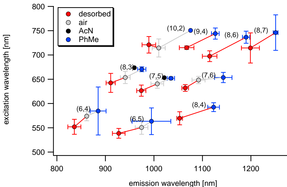
Fig. 17: The figure shows the shift of the excitonic transition energies to lower energies upon the transfer from air to toluene. The nanotubes in air are clearly assignable into two classes that experience two different dielectric surroundings.
