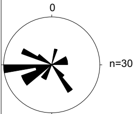
Western and central Tsarabis Fm. Palaeo-currents: 10 ° classes
