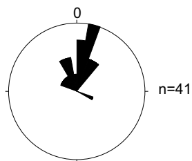
Eastern Verbrandedberg Fm. Palaeo-currents: 10 ° classes
