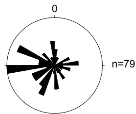
Tsarabis Fm. (general) Palaeo-currents: 10 ° classes
