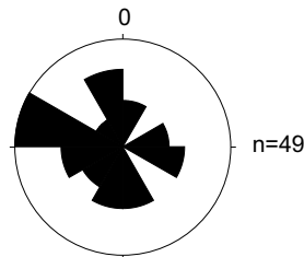
Eastern Tsarabis Fm. Palaeo-currents: 30 ° classes
