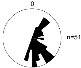
Upper Aeolian Unit (general) Dune foreset dip-directions: 10 ° classes
