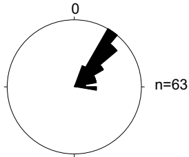
Main Aeolian Unit (general) Dune foreset dip-directions: 10 ° classes
