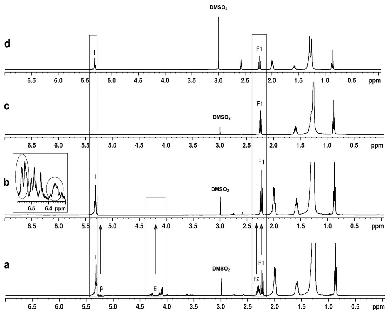
Fig. 2 Stacked plot ^1\text{H} NMR Spectra at \delta = 0.00\text{--}7.00 ppm (from bottom to top) of a RFO (100 mg), b hydrolyzed RFO (85 mg) with enlargement region of \delta = 6.20\text{--}6.80 ppm, c palmitic Acid standard, and d oleic acid standard
