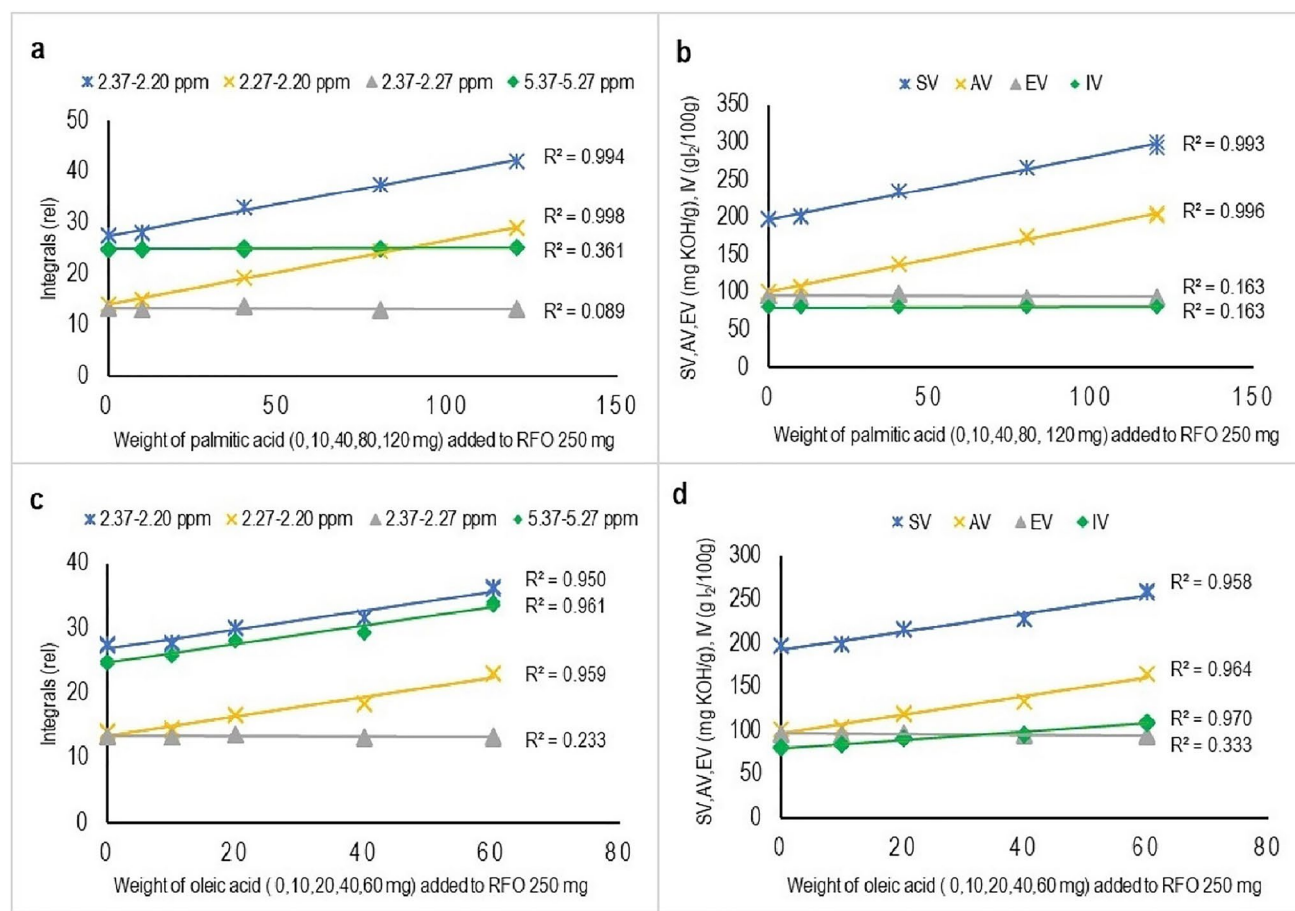
Fig. 5 a Correlation between RFO with palmitic acid addition versus Integral of ^1\text{H} NMR RFO ( \delta=5.37\text{--}5.27 ppm, \delta=2.37\text{--}2.27 ppm, \delta=2.27\text{--}2.20 ppm, and \delta=2.37\text{--}2.20 ppm) and b correlation between RFO with palmitic acid addition versus SV, AV, EV, and IV by qNMR calculation. c Correlation between RFO with oleic
