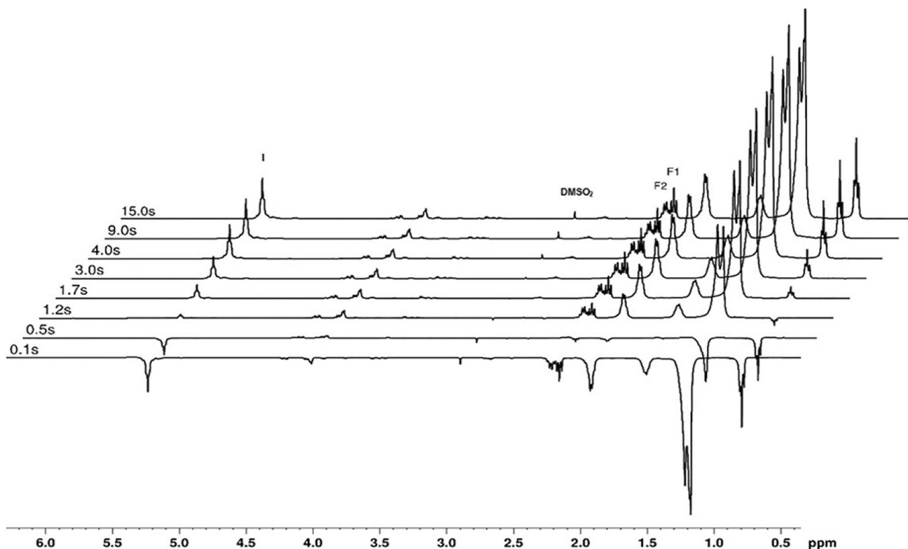
Fig. 3 400 MHz 1 H NMR; an inversion-recovery pulse sequence of experiments used to measure the values of T1 for the protons of RFO in CDCl 3 :DMSO-d 6 (5:1, v/v), flip angle 180°—τ—90° was applied
