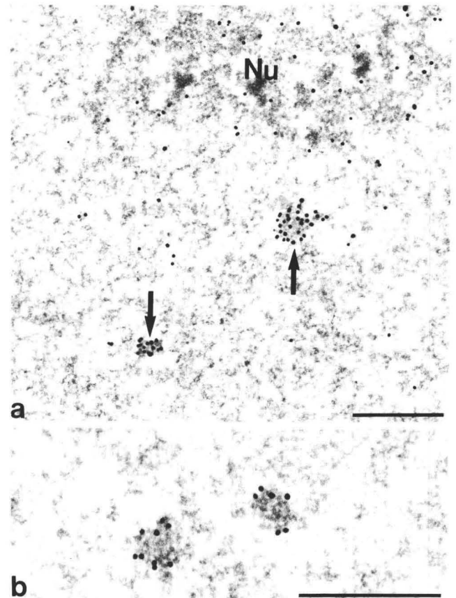
FIGURE 8 Identification of the small protein S1-containing nucleoplasmic entities described in Fig. 4 by electron microscopic immunolocalization in hepatocyte nuclei of regenerating rat liver (these specimens have been fixed with formaldehyde after incubation with the primary antibody). The survey electron micrograph (a) shows a part of the nucleolus (Nu) and two of the protein S1-containing nucleoplasmic aggregates (arrows) which are heavily labeled with gold particles of 20 nm diam. At higher magnification (b), these aggregates appear as distinct structural entities of relatively high electron density, most of them with diameters ranging from 0.1 to 0.3 \mu\text{m} , and display a finely granular composition. Bars, 0.5 \mu\text{m} . (a) \times 33,000 ; (b) \times 54,000 .
