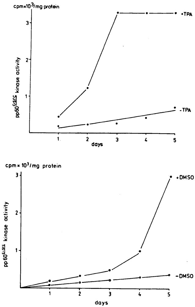
Fig. 3. Kinetics of pp60 c-src kinase activity in HL-60 cells after induction of differentiation with TPA (upper part, +TPA) and with DMSO (lower part, +DMSO). In control experiments untreated sister cultures were tested (-TPA, -DMSO). Experimental details as described in Figure 1.
