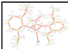
Fig. 1. The molecular structure of title compound. Displacement ellipsoids are drawn at the 30% probability level. The H atoms are presented as a small spheres of arbitrary radius.
