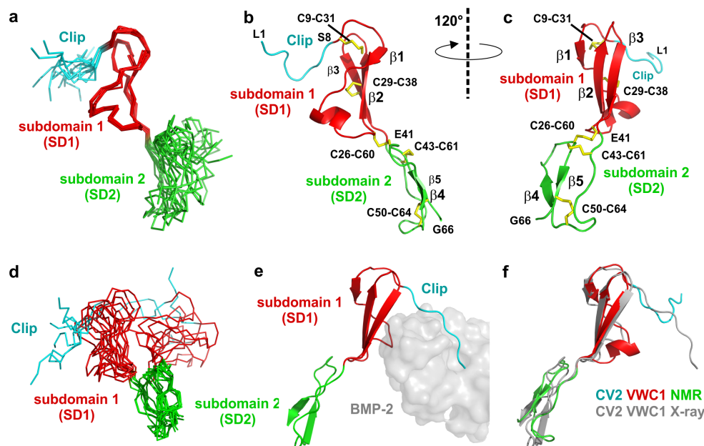
Figure 2. (a) Structure ensemble of ten NMR structures of CV2 VWC1 aligned to subdomain 1. (b) Ribbon plot of the NMR structure of CV2 VWC1, subdomain boundaries for the Clip segment (L1 to S8) and the subdomains 1 and 2 are indicated, disulfide bonds are shown as sticks. (c) As in (b) but rotated around the y-axis by 120°. (d) Structure ensemble as in (a) but aligned on the backbone atoms of subdomain 2. (e) CV2 VWC1 bound to BMP-2 (PDB entry 3BK3), the VWC1 domain is shown as ribbon plot, BMP-2 is shown as semi-transparent van der Waals surface in grey. The Clip segment folds into the BMP type I receptor-binding site, subdomain 1 is attached to the BMP type II receptor site. (f) Structure alignment of CV2 VWC1 in its bound (indicated in grey) and unbound conformation (labeled CV2 VWC1 NMR).
