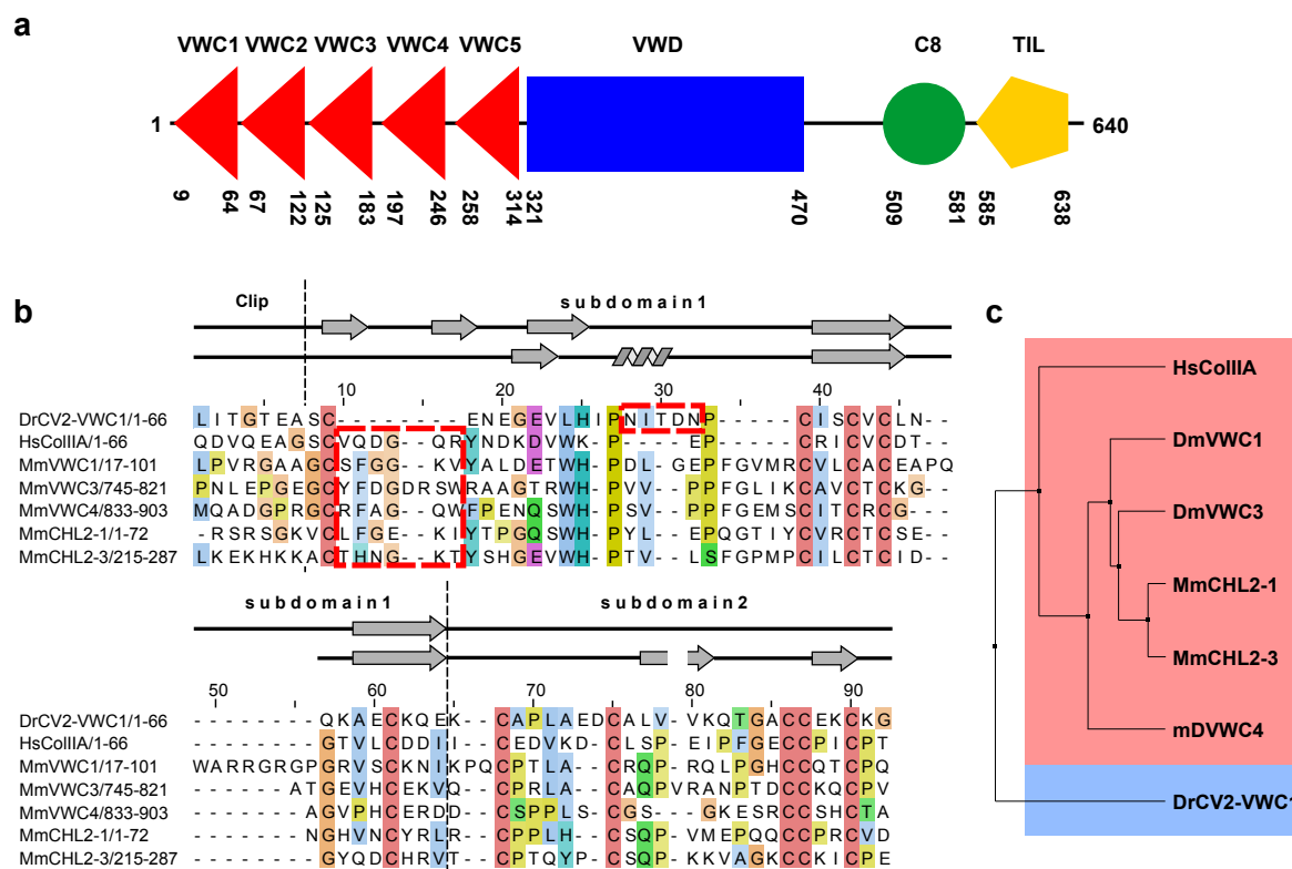
Figure 5. (a) Architecture of the BMP modulator Crossveinless 2. The VWC domains 1 – 5 are indicated by red triangles, the VWD domain by a blue rectangle, the C8 and the TIL domain by a green circle and an orange pentagon. The amino acid boundaries of the protein domains are obtained from the PFAM and SMART database using the amino acid sequence of mature Danio rerio Crossveinless 2. (b) Sequence alignment based on a structure comparison of the VWC domains of Danio rerio CV2 (VWC1) and human procollagen IIA (UniProt code P02458) showing that VWC domains might cluster into two classes. For comparison other VWC domains from modulator proteins of the Chordin family are shown (MmVWC1, 3, 4: Mus musculus Chordin VWC domains 1, 3 and 4, UniProt code Q9Z0E2; MmCHL2-1, 3: Mus musculus Chordin-like 2 VWC domains 1 and 3, UniProt code Q8VEA6). Architectural features of the CV2 VWC1 domain are indicated; secondary structure elements as present in the NMR structures of procollagen IIA VWC (upper line) and CV2 VWC1 (lower line) are shown. The boxes marked by red stippled lines indicate the two discriminatory sequence features leading to the differing structures observed for both VWC domains. (c) Phylogenetic analysis using the sequence alignment shown in (a).
