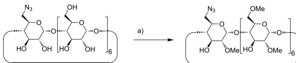
Scheme 1: Synthesis of azido functionalized DIMEB 1a . a) \text{Ba}(\text{OH})_2 \cdot 8\text{H}_2\text{O}/\text{BaO}/\text{Me}_2\text{SO}_4
