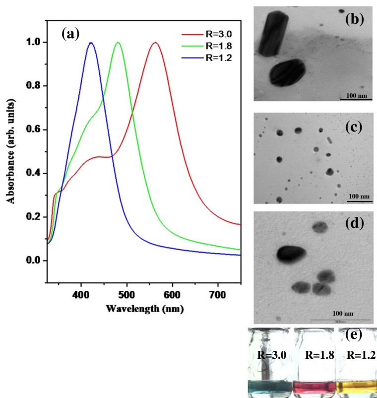
Figure 2 UV-visible spectrum of synthesized silver nano nanorods solutions, NR1, NR2, and NR3 of different aspect ratios (a) TEM micrograph of NR1 (b) TEM micrograph of NR2 (c) TEM micrograph of NR3 (d) and a picture of synthesized nanorods solutions (e).
