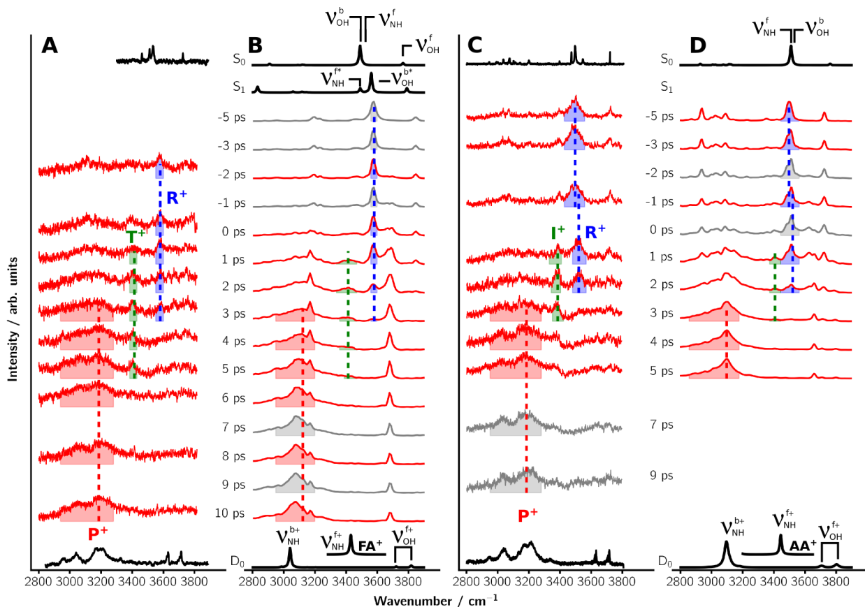
Figure 2: ps-TRIR spectra of \text{FA}^+ - \text{W} from experiment (A) and MD simulations (B) compared to ps-TRIR spectra (C, 36 ) and MD simulations (D, 37 ) of \text{AA}^+ - \text{W} . The S_0 , S_1 and D_0 spectra are stationary IR spectra of the CO-bound ( S_0 , S_1 ) and NH-bound ( D_0 ) isomers in the neutral and cationic states determined by nanosecond lasers (A, 39 C) and DFT harmonic frequency calculations for the optimized structures (B, D). The inset in the D_0 spectra shows the NH stretch mode for bare \text{FA}^+ and \text{AA}^+ . The highlighted areas indicate the signals uniquely attributed to the CO-bonded isomer (blue, \text{R}^+ ), the intermediate or transient structure (green, \text{I}^+ / \text{T}^+ ), where water is bound neither to the NH nor the CO site, and the NH-bound geometry (red, \text{P}^+ ). The gray shaded spectra denote signals which are not recorded within the experiment or are out of scope of the simulation time, respectively.
