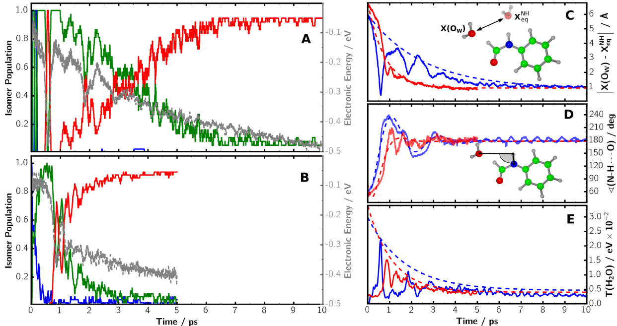
Figure 4: Left panels: Averaged populations of the FA + - W (A) and AA + - W (B) ensembles, with the CO-bound isomer (blue), the transient or intermediate structure (green), and the NH-bound isomer (red) as a function of simulation time. The gray dashed line shows averaged electronic energy from the MD simulations. Right panels: (C) Averaged distance of the water oxygen (O W ) from its NH-bound equilibrium geometry, (D) averaged angle between the N-H bond of the peptide and O W , and (E) averaged kinetic energy of water along the trajectories of FA + - W (blue) and AA + - W (red). The dashed lines in (C) and (E) are exponential fits with respect to the maxima of the curves. For (D) a damped harmonic oscillator was fitted to the curve.
