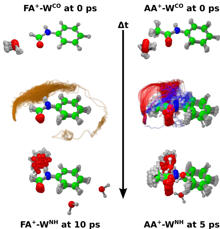
Figure 5: Trajectories of the ionization-induced water migration derived from the \text{FA}^+ - \text{W} (left, 40 trajectories) and \text{AA}^+ - \text{W} (right, 50 trajectories) MD simulations, starting from the CO-bound isomer (top row) and ending at the NH-bound isomer (bottom row) at 10 ps and 5 ps after ionization, respectively. The yellow curve for \text{FA}^+ - \text{W} indicates the in-plane migration path of water. The out-of-plane pathways for \text{AA}^+ - \text{W} correspond to the slow (blue) and fast (red) migration channels, respectively. 37
