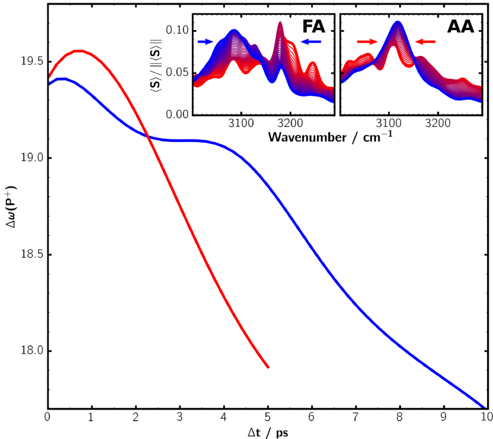
Figure 6: Average peak width \Delta\omega of the product band ( \nu_{NH}^{b+}, P^+ ) calculated for \text{FA}^+ - \text{W} (blue) and \text{AA}^+ - \text{W} (red) from the simulated ps-TRIR spectra (Fig. 2B and 2D). The peak width has been calculated as \Delta\omega = (\omega_2 - \omega_1)^{-1} \int_{\omega_1}^{\omega_2} d\omega [\langle\omega^2\rangle - \langle\omega\rangle^2]^{\frac{1}{2}} \frac{\langle S(\omega, \Delta t) \rangle}{\|\langle S(\omega, \Delta t) \rangle\|} , with \omega_1 = 3000 \text{ cm}^{-1} and \omega_2 = 3300 \text{ cm}^{-1} . The insets show the normalized band of \text{FA}^+ - \text{W} and \text{AA}^+ - \text{W} , respectively.
