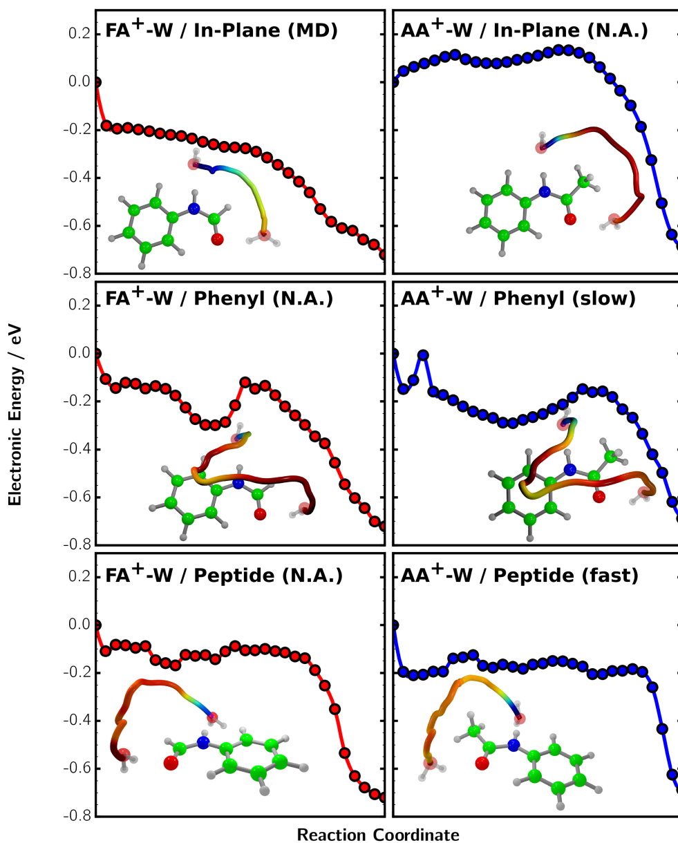
Figure 3: Minimum energy paths derived from the nudged elastic band method of FA – W + (left) and AA – W + (right) for the migration of water from the CO to the NH site along the in-plane path (top row), above the phenyl ring (middle row), and above the peptide bond (bottom row). The insets illustrate the path of water, whereby the color encodes the energy at the point of the path. N.A. indicates the pathways not detected by the experiment and the simulations.
