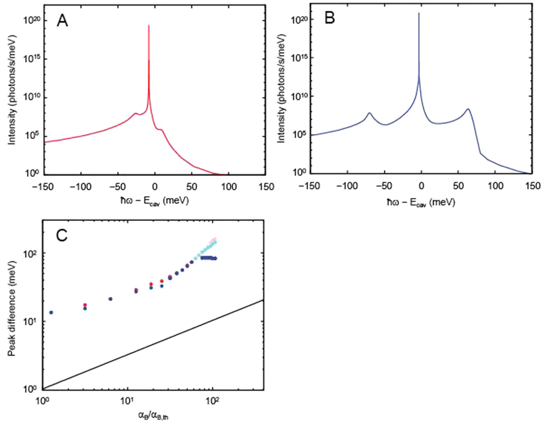
Figure 4. Numerical results for the spectral properties. (A,B) Calculated photoluminescence spectrum I_{SS}^{inc}(\omega, \mathbf{q} = 0) at \mu_B - E_{LP} = 5 meV ((A), low excitation density) and 80 meV ((B), high excitation density) indicated by the arrows in Fig. 5B. The experimental energy separation between the two peaks are an order of magnitude smaller than the calculated values. This discrepancy may be caused by dephasing and polariton–polariton scattering processes not taken into account in our theory. (C) Energy separation between the main peak and the side-band peaks as a function of the pumping strength \alpha_B \equiv \mu_B - E_{LP} . In order to compare the results with the experiments, \alpha_B is again normalized by its threshold value \alpha_{B,th} \equiv \mu_{B,th} - E_{LP} (= 1.64 meV). The blue (red) points denote the difference in energy positions between the higher-energy (lower-energy) sideband and the main peak, the transitions of which are indicated by the blue (red) and black arrows in Fig. 3. We note that, under the lasing conditions, the calculated spectra exhibit two additional weak peaks (not shown), corresponding to the aqua and pink transitions in Fig. 3(b). We therefore plot the energy separation between the main peak and the two additional peaks by aqua and pink in panel (C). The PL intensities of the two additional peaks are smaller than that of the high-energy peak by blue. Therefore, the discussion about the existence of those peaks are not given in the text. The black solid line is a guide for the eye proportional to (\alpha_B/\alpha_{B,th})^{1/2} .
