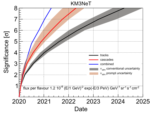
Figure 1. Significance as a function of time for the detection of a diffuse flux of neutrinos corresponding to the signal reported by IceCube, for cascade-like events (red line) and track-like events (black line). The black and red bands represent the uncertainties due to the conventional and prompt component of the atmospheric neutrino flux, respectively. The blue line indicates the result of the combined analysis.
