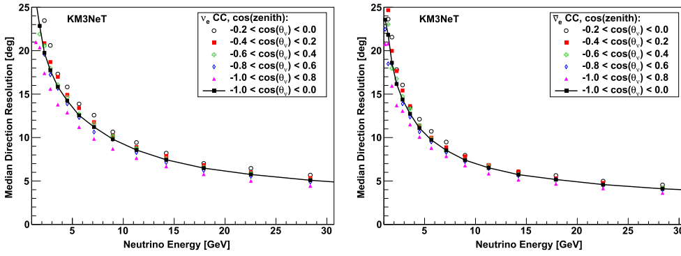
Figure 80. Median neutrino direction resolution (angle between reconstructed direction and neutrino direction) as a function of neutrino energy for different true neutrino cos(zenith) ranges, where \cos(\text{zenith}) = -1 means vertical up-going and \cos(\text{zenith}) = 0 means horizontal. The black line corresponds to up-going neutrinos weighted according to the Bartol flux model. \nu_e CC (left) and \bar{\nu}_e CC (right).
