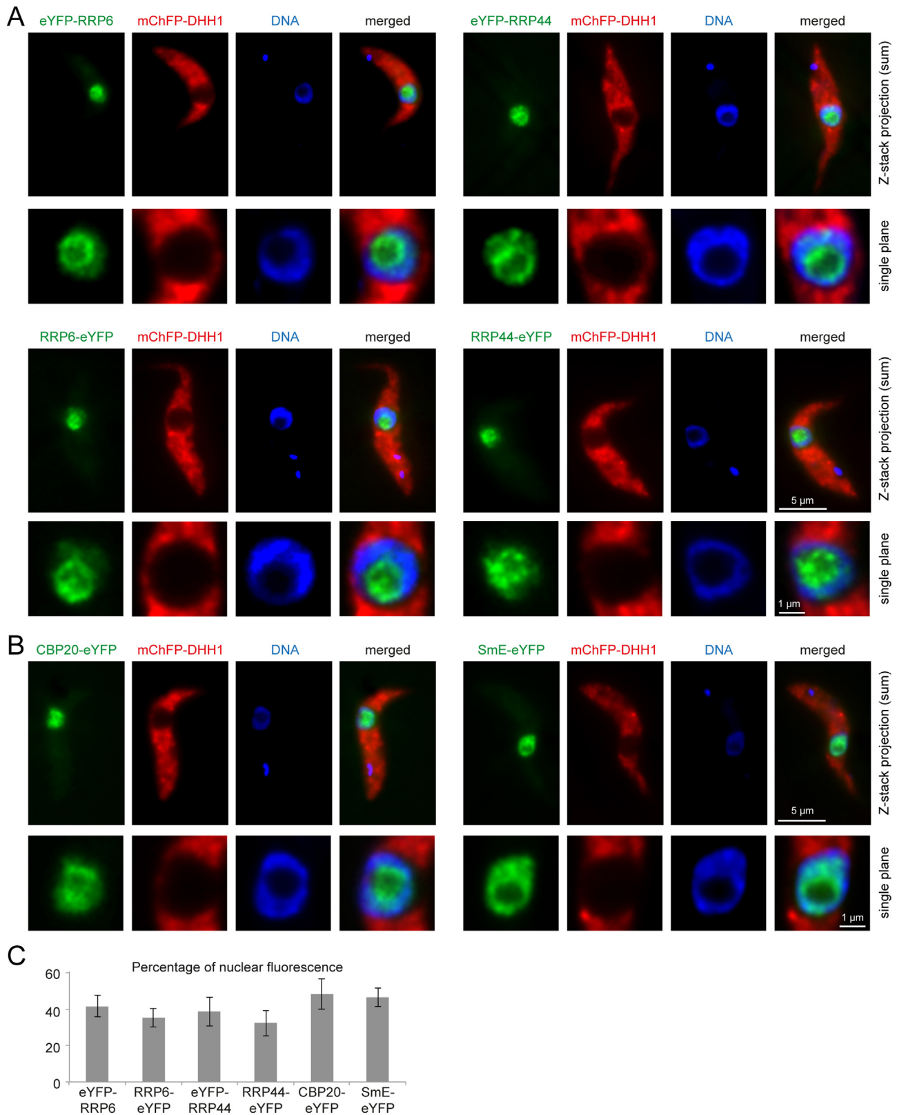
Fig. 2. Localization of N and C-terminal eYFP fusions of RRP6 and RRP44. Two nuclear control proteins (CBP20 and SmE) served as controls. (A + B) Z-stacks (100 images, 100-nm spacing) were recorded with a custom-built TILL Photonics iMIC microscope equipped with a 100 \times , 1.4 numerical aperture objective (Olympus, Tokyo, Japan) and a sensicam qe CCD camera (PCO, Kehlheim, Germany); deconvolved using Huygens Essential software (SVI, Hilversum, The Netherlands). For each cell line, one representative fluorescent cell is shown as a Z-stack projection (method sum slices). In addition, the nucleus of a deconvolved single plane image is shown enlarged. (C) For each eYFP fusion protein, the percentage of fluorescence in the nucleus was quantified from the Z-stack projections of deconvolved images of at least 16 cells. Error bars indicate standard deviations.
