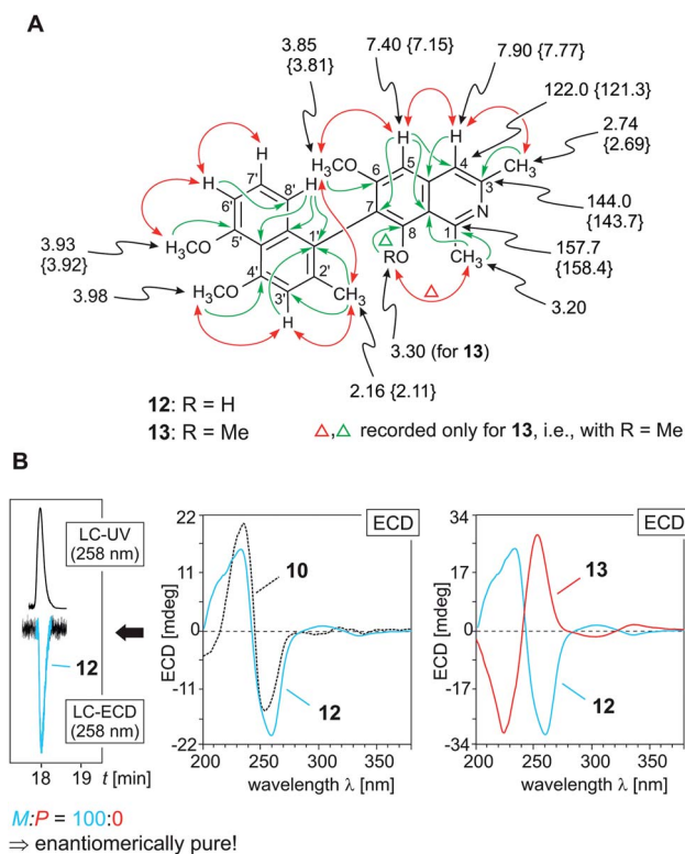
Fig. 3 (A) Selected ^1\text{H} and ^{13}\text{C} NMR data (in methanol- d_4 , \delta in ppm), HMBC (single green arrows), and NOE interactions (double red arrows) of ancistrobreveines A ( 12 ) and B ( 13 ); the values of 13 that are different from those of 12 are given in {}; (B) HPLC-ECD analysis on a chiral phase (Lux Cellulose-1) giving only one peak, revealing that in A , abbreviatus 12 occurs in an enantiopure form (left), and assignment of the absolute axial configuration of 12 (center) and 13 (right) by comparison of the ECD spectrum of 12 with that of the 7,1'-coupled known M -configured ent -dioncophylleine A ( 10 ; for its structure, see Fig. 1), and by comparison of the ECD spectrum of 13 with that of 12 .
