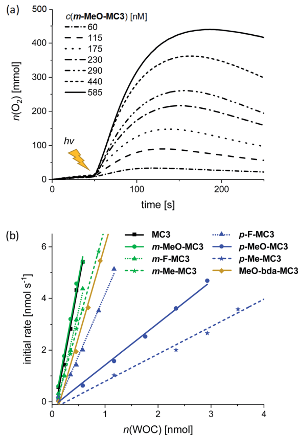
Fig. 5 (a) Concentration-dependent oxygen evolution curves of m -MeO-MC3 in MeCN/H 2 O 1 : 1 (pH 7, phosphate buffer), c (PS) = 1.5 mM, c (Na 2 S 2 O 8 ) = 37 mM. The lighting symbol indicates the start of sample irradiation at t = 50 s. (b) Initial rates of all macrocycles with linear regression for the determination of averaged TOF.
