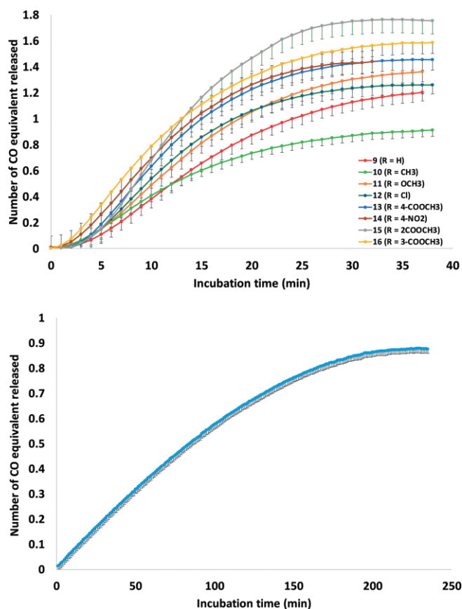
Figure 6. CO release profiles of 9–16 in DMSO/water (1:10 v/v) analyzed with a commercial CO sensor system under constant illumination with LED light at 468 or 525 nm (top) during the initial 30 min and (bottom) upon extended illumination of 14 at 525 nm for up to 4 h. All data are expressed as mean \pm SD ( n = 3 ).
