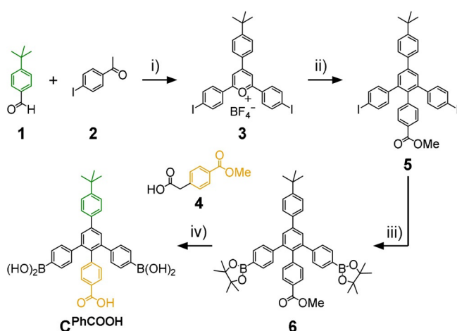
Scheme 1. Modular synthesis of diboronic acid C PhCOOH : i) \text{BF}_3 \cdot \text{OEt}_2 , 100 °C, 2 h, 38%; [27] ii) 4^{[29]} /NaOH, MeOH, 30 min, then \text{Ac}_2\text{O} , 160 °C, 2 h, 55%; [28] iii) \text{B}_2\text{pin}_2 /KOAc/Pd(dppf) \text{Cl}_2 , DMF, reflux, 2.5 h, 71%; iv) \text{BBr}_3 , \text{CH}_2\text{Cl}_2 , 0 °C → rt, 3.75 h, 76%.
