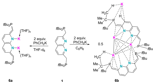
Scheme 4. The synthesis of 6a and 6b by two-fold deprotonation.
