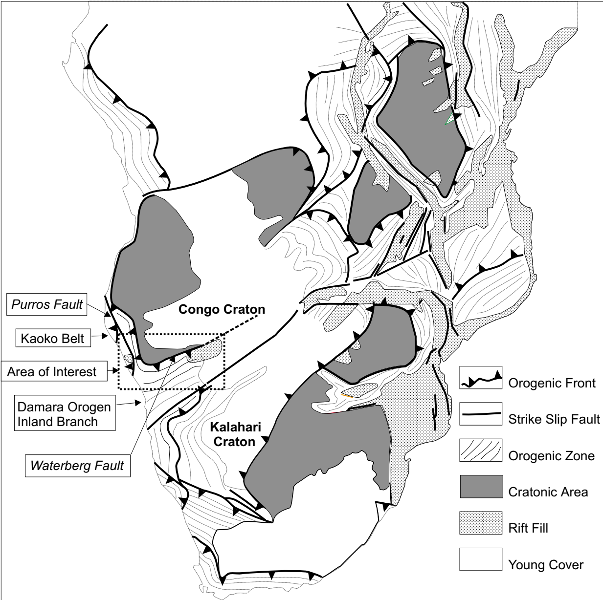
Precambrian Cratonic and Orogenic Zones in Southern Africa
