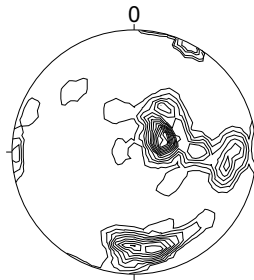
Poles to fault planes Faults within the Korne Mbr. and Mixed Aeolian-Fluvial Unit at Krone Farm
