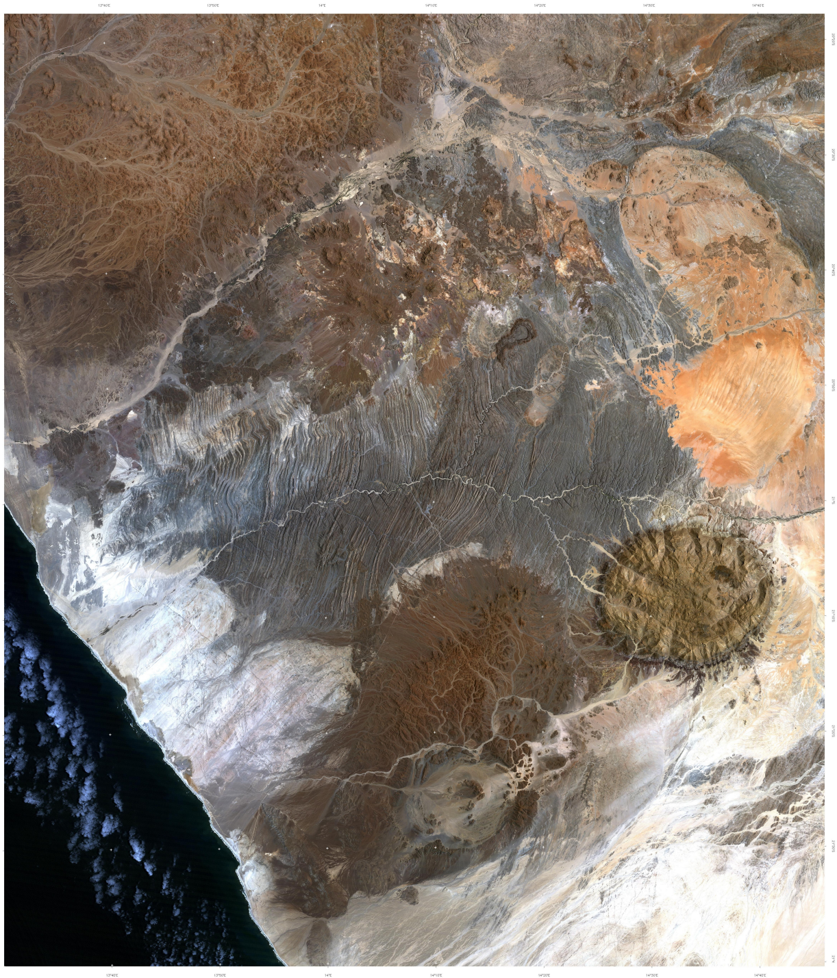
Landsat TM 5 image showing the southern Etendeka, Huab River, Ugab River, Brandberg, Messum Crater and Albin Ridge.
