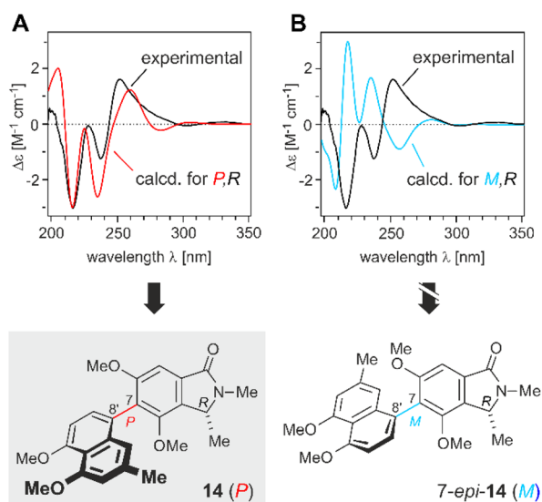
Fig. 4 Assignment of the absolute configuration of ancistrobrevoline A (14) by comparison of its experimental ECD spectrum (in black, taken in methanol) with the ones calculated (A) for the (1 R ,7 P )-isomer (ECD curve in red) and (B) for 1 R ,7 M (in pale blue) using TD \omega B97XD3/def2-TZVP//B3LYP-D3/def2-TZVP.
