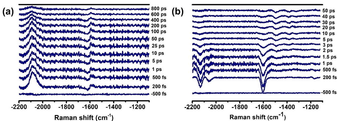
Figure 6. URLS spectra of DACN-DPA in (a) n -hexane, and (b) MeCN at different delay times.
