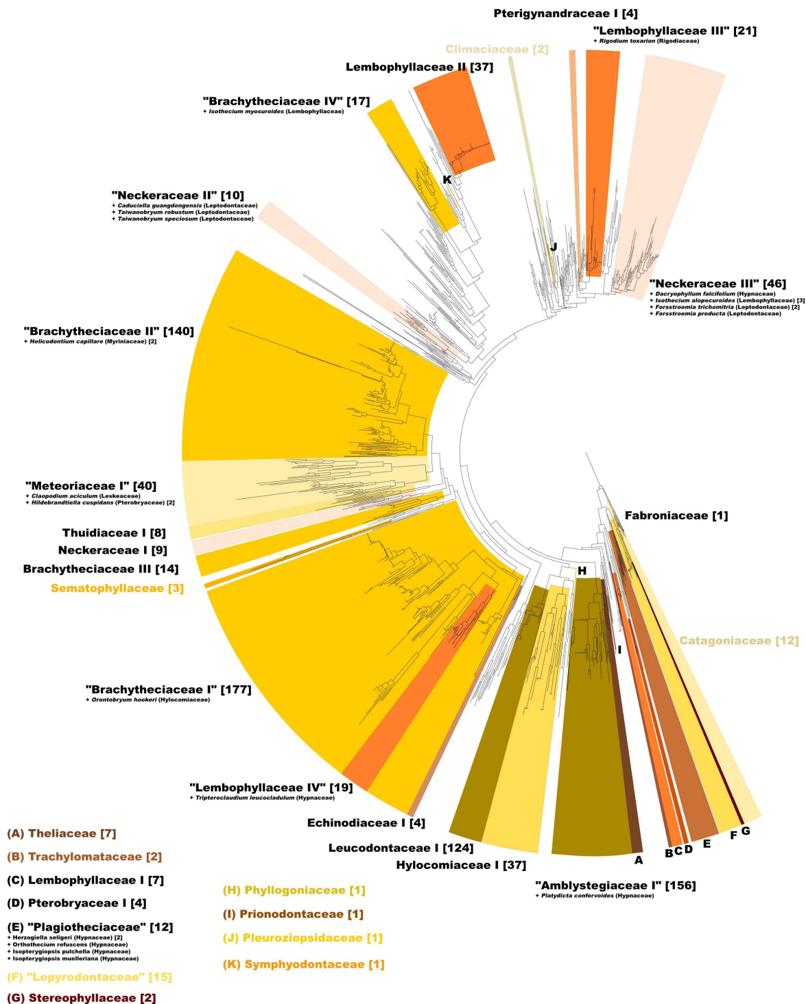
Figure 2 Neighbor-Joining tree of 1,634 hypnalian sequence-structure pairs. Mono- and paraphyletic clades are highlighted and labeled. Paraphyletic clades are indicated by quotes. A colored label denotes a clade as a complete monophylum containing each used sequence of this family. It is possible that some clades are labeled with "I", although there is no corresponding clade "II". In this case the missing sequences are spread in the non-monophyletic (uncolored) areas of the tree. Numbers in squared parentheses show the quantities of sequences in the specific clade. An apparently small clade can yet contain many sequences. In this case different sequence-structures of the same species built a monophylum and were collapsed for reasons of clarity and comprehensibility. Collapsed clades are marked by triangles instead of lines within the tree.
