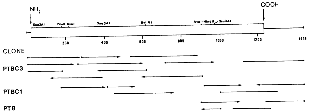
Fig. 1. Strategy for sequencing full-length cDNA coding for the spinach chloroplast phosphate translocator subcloned into the plasmid vector pT7T3. Sequencing was carried out by the dideoxy chain termination method (Sanger et al. , 1977) using T7 and T3 primers, dGTP/7-deaza-dGTP and [ \alpha - 35 S]dATP as radioactive label. Some regions of the cDNA were sequenced using exonuclease III/S1 nuclease treated cDNA clones (PTBC3, 1439 bp; PTBC1, 1266 bp; PT8, 544 bp) which had been digested with Bam HI and Pst I (Henikoff, 1984). In addition, the insert of PTBC3 was digested with different restriction enzymes ( Ava II, Pvu II, Sau 3AI, Bst NI) as indicated and subcloned into the Sma I site of pT7T3. The horizontal arrows represent the directions on length of the sequences determined. The positions of the amino- and carboxyl-termini are indicated by arrows.
