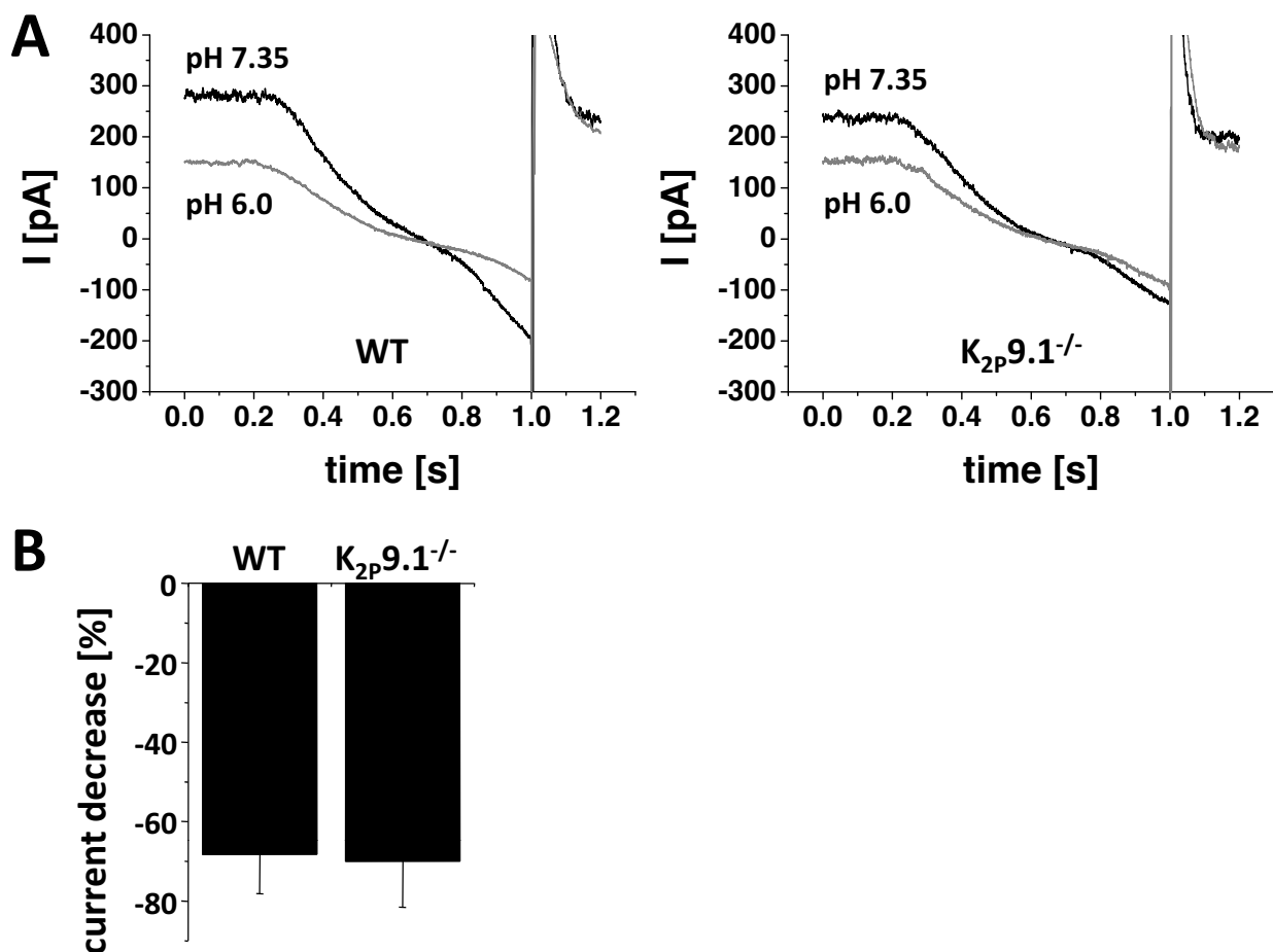
Figure 2 pH dependence of the standing outward currents in K_{2p9.1}^{-/-} neurons shows no difference compared to wildtype mice (pH 7.35 T pH 6.0). (A) Ramp currents under control conditions (pH 7.35) and after extracellular acidification (pH 6.0) in wildtype (WT; left panel) and K_{2p9.1}^{-/-} mice (right panel). (B) Bar graph representation of current reduction after extracellular pH lowering in wildtype (WT) and K_{2p9.1}^{-/-} mice.
