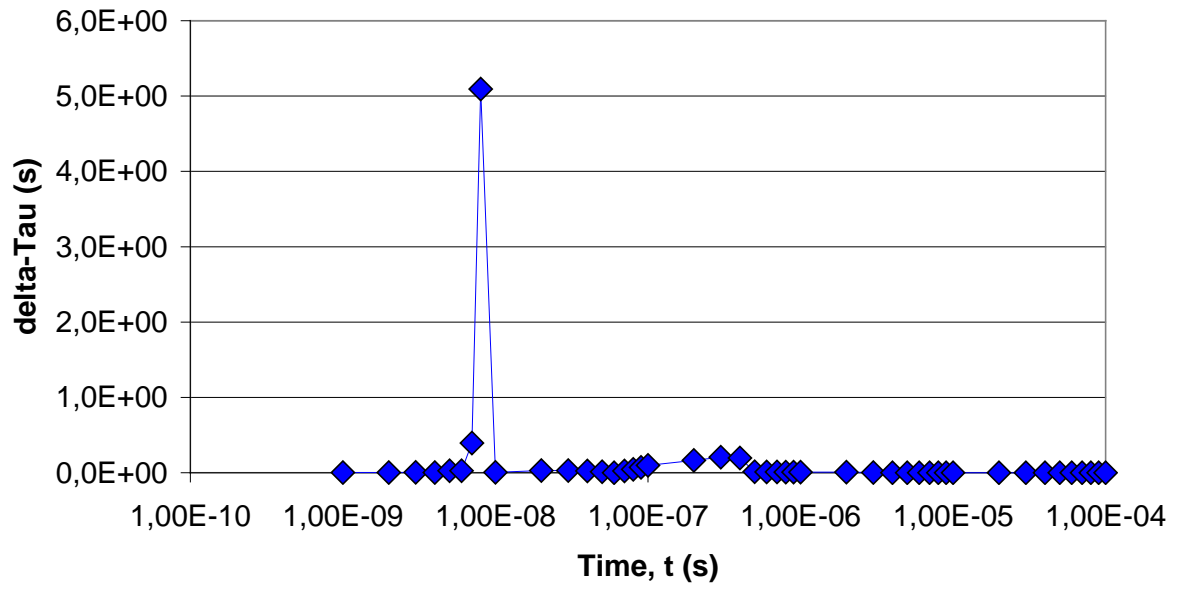
Time interval, delta-Tau, near central front positions of NbTi-filament, vs. real time, t
