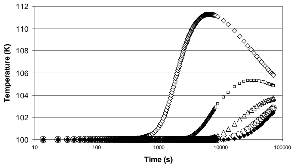
Temperatures at different optical thickness after absorption of two radiative pulses at the position x = 0
