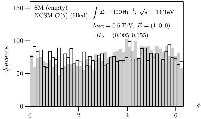
Figure 3.9: Monte Carlo simulation for the azimuthal dependence of the process pp \rightarrow e^+e^-\gamma at the LHC.
