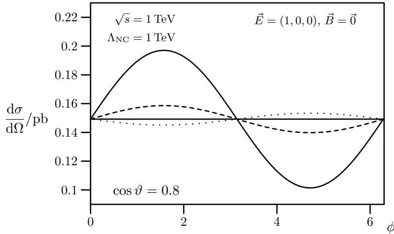
Figure 3.11: Azimuthal dependence of the cross section, with different values for the TGB couplings: K_1 = (-0.333, 0.035) (solid), K_5 = (0.095, 0.155) (dotted) and K_0 = (0.0, 0.0) (dashed).
