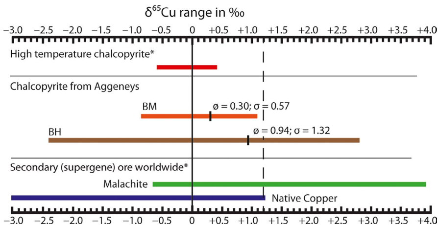
FIGURE 4 \delta^{65}\text{Cu} values of chalcopyrite from the Broken Hill and Black Mountain deposit at Aggeneys compared to terrestrial high-temperature chalcopyrite and supergene ores worldwide. * = Ikehata et al. (2011). Broken line = Supergene average (Mathur & Fantle, 2015) [Colour figure can be viewed at wileyonlinelibrary.com ]
