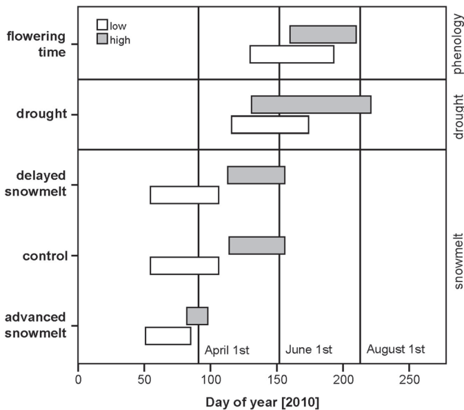
Fig. 1. Range in the date of snowmelt (advanced snowmelt, control, delayed snowmelt), duration of drought treatment, and flowering time of all species over the lower (600–1300 m) and the higher (1300–2000 m) altitudinal gradient in 2010.
